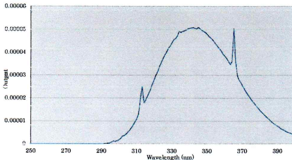
340 nm F40T12 Lamp Output
